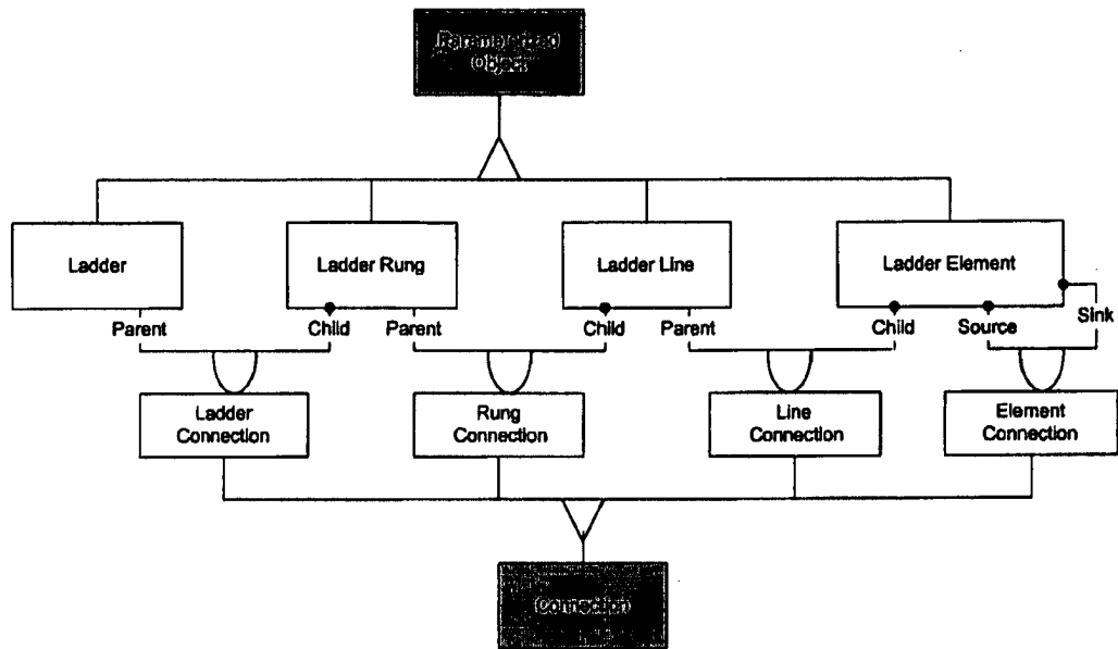
Figure 96 - Ladder Objects
